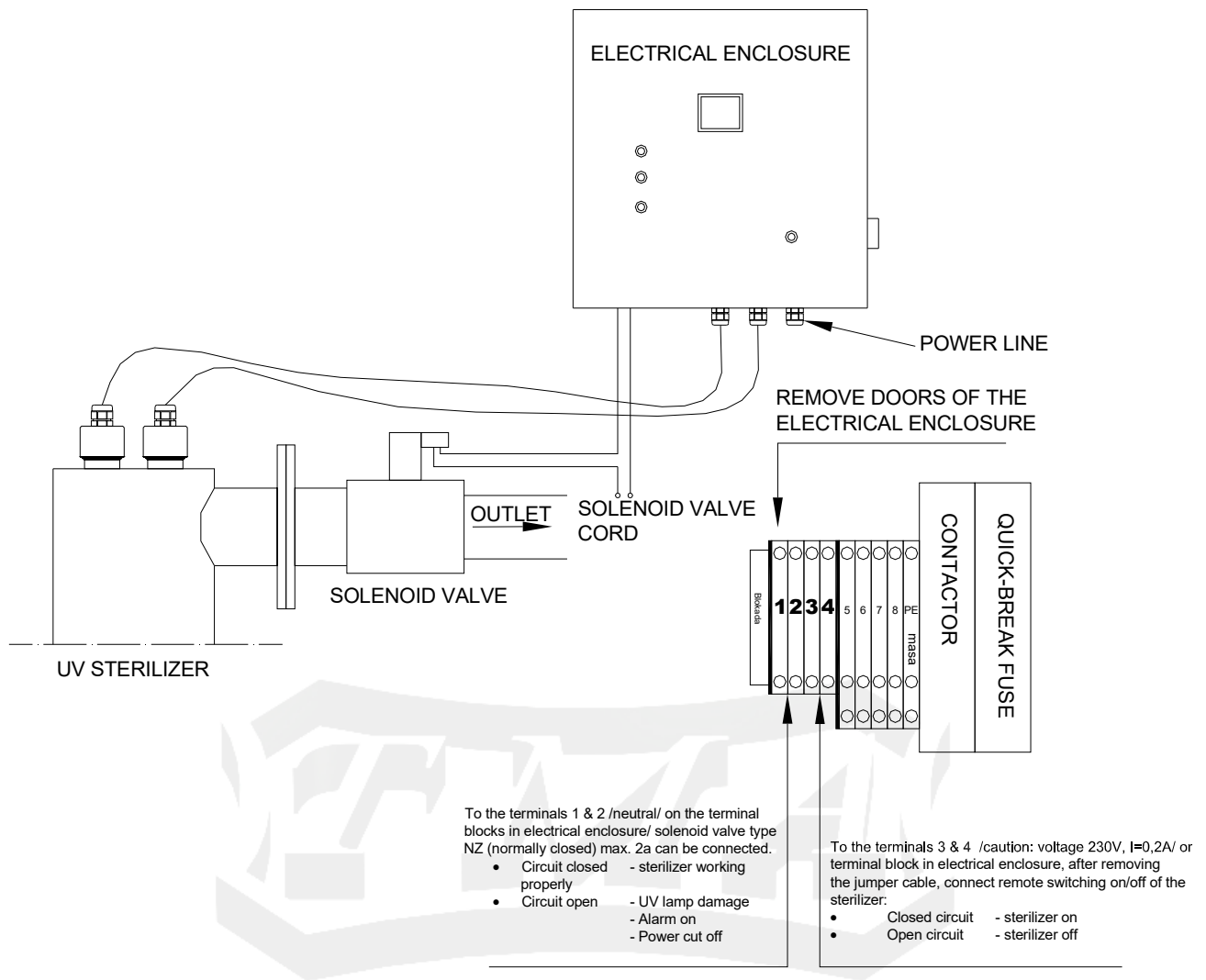
AP-POOL-N 2 - Diagram for solenoid valve, alarm signal and outside connection of the device.
